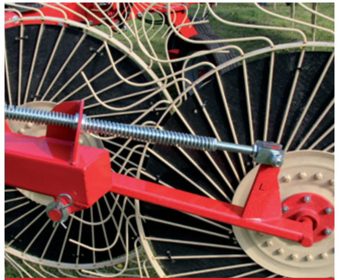
Independent rake wheel arms.
